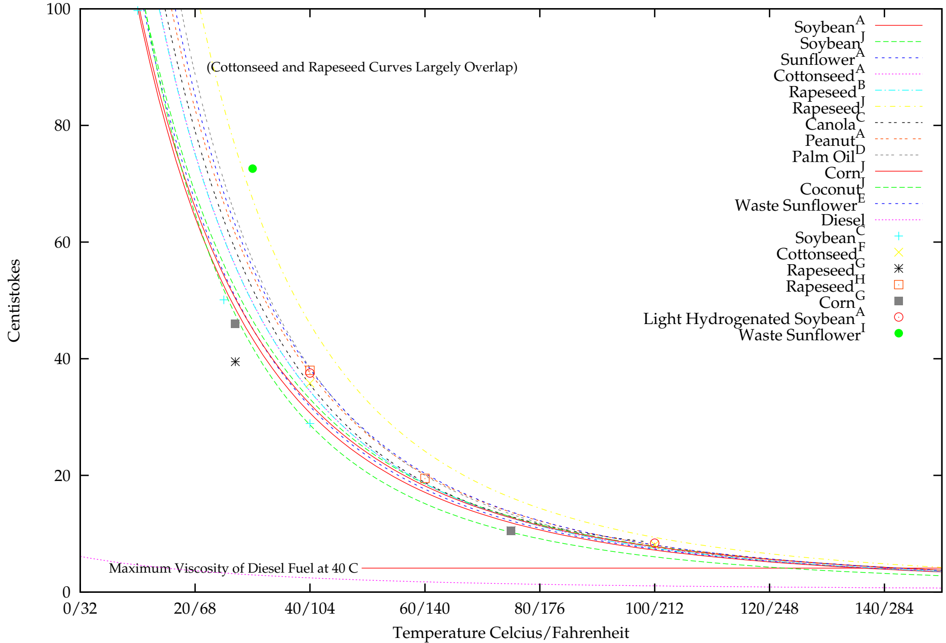
Figure A: Temperature Dependence of Viscosity of Various Vegetable Oils
